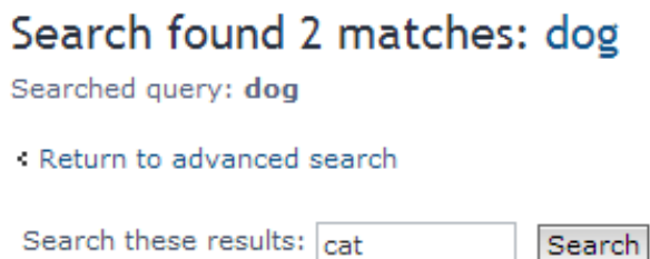
Figure 5.9. Search refinement
